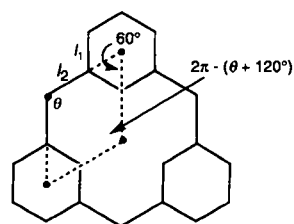
Scheme 8: Projection of 3-fold helix along the polymer axis (actual rather than projected angles and distances are shown).
