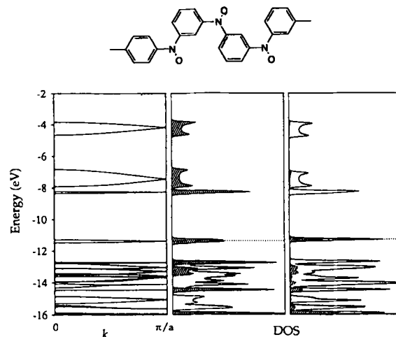
Fig. 12. Band structure and DOS (center) of the planar polymer with nitroxide ( NO' ) radicals coupled through a meta -phenylene unit. The projection of the first DOS (center) is the contribution from \pi bands. That in the second DOS (right) shows the contribution just from the pseudo- \pi orbitals at the radical centers (N and O) of the 3-fold helical structure.
