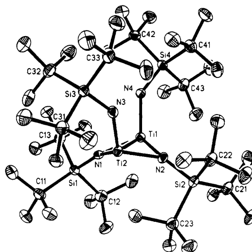
Figure 1. Molecular view of [(\text{tBu}_3\text{SiNH})\text{Ti}]_2(\mu\text{-NSi}^t\text{Bu}_3)_2 ( 17 ).
