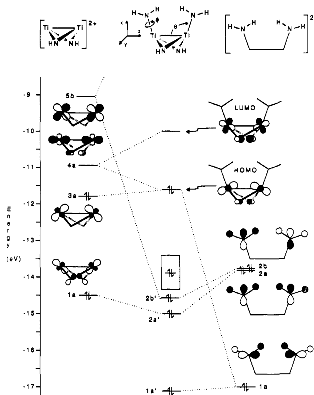
Figure 5. Truncated molecular orbital diagram of [(H 2 N)Ti] 2 ( \mu -NH) 2 (17''), a model complex of [( t Bu 3 SiNH)Ti] 2 ( \mu -NSi t Bu 3 ) 2 (17).
