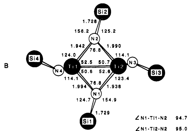
Figure 2. Skeletal views of [(\text{tBu}_3\text{SiNH})\text{Ti}]_2(\mu\text{-NSi}^t\text{Bu}_3)_2 ( 17 ). Bond distances are in angstroms and bond angles are in degrees.
