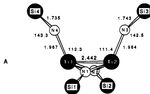
Figure 1. Molecular view of [(\text{tBu}_3\text{SiNH})\text{Ti}]_2(\mu\text{-NSi}^t\text{Bu}_3)_2 ( 17 ).
