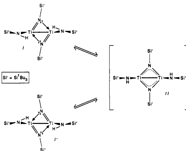
Figure 3. Interconversion of two plausible resonance structures of [(\text{Bu}_3\text{SiNH})\text{Ti}]_2(\mu\text{-NSi}^i\text{Bu}_3)_2 ( 17 ).
