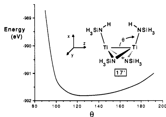
Figure 4. Energy (eV) of [(\text{H}_3\text{SiNH})\text{Ti}]_2(\mu\text{-NSiH}_3)_2 ( 17' ), a model complex of [(\text{Bu}_3\text{SiNH})\text{Ti}]_2(\mu\text{-NSi}^i\text{Bu}_3)_2 ( 17 ), as a function of both Ti-Ti-N amide angles, each defined by \theta ( 90^\circ \leq \theta \leq 190^\circ ).
